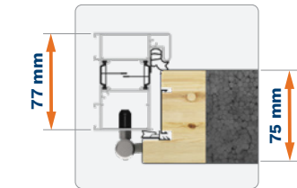
ALUTHERM 75 aluminium frame
