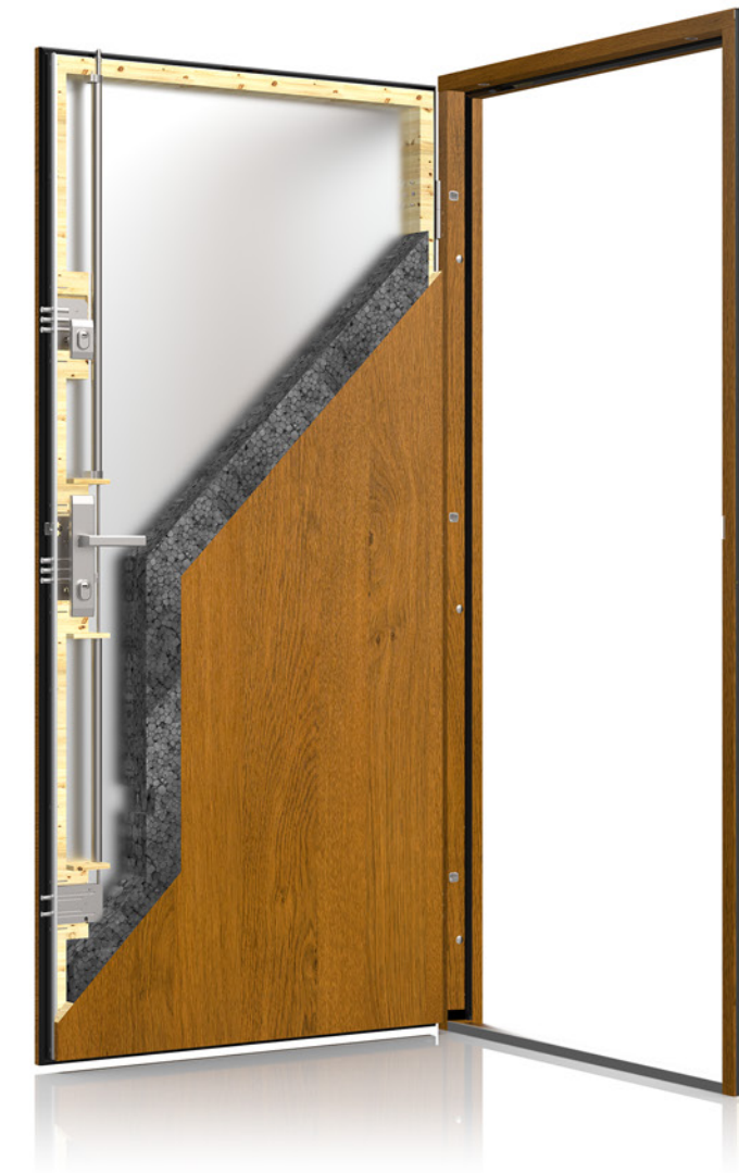
Adjustable keep enables smooth adjustment of the contact force of door and seals
